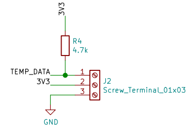
OPTIONAL DS18B20 TEMPERATURE SENSOR
