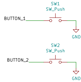
CALIBRATION PUSHBUTTONS C&K PN KMR742NG LFS Digikey CKN10689CT-ND
