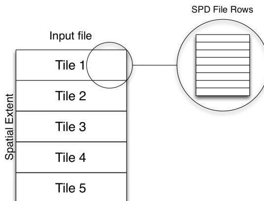
Figure 4.1: spdtranslate tiling.
