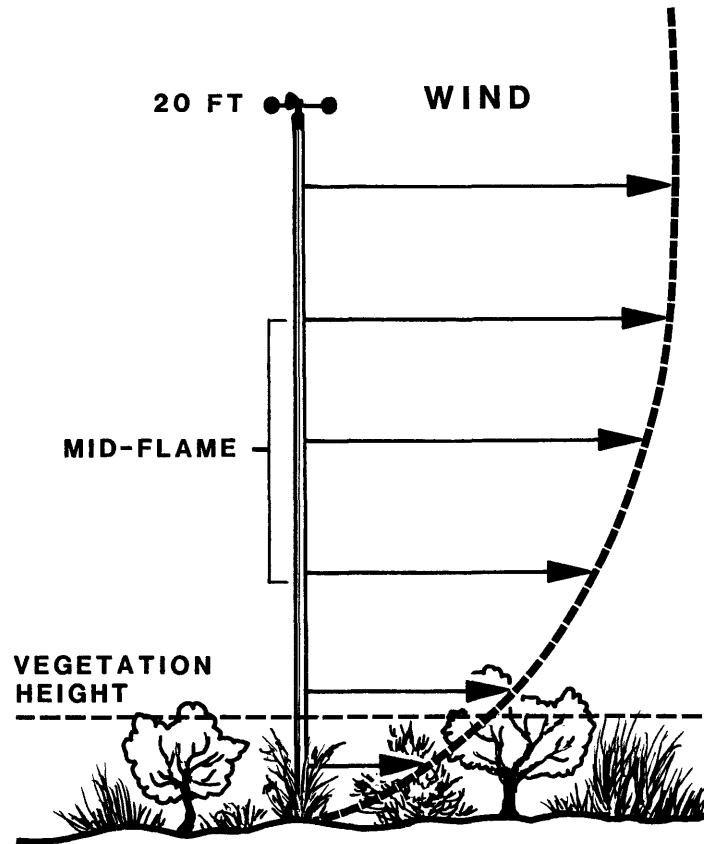
Figure 7.—Near-surface wind profile.
