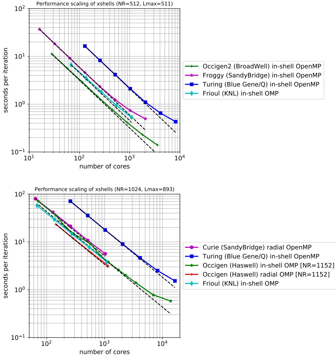
Figure 1.1: Performance scaling of XSHELLS, on french supercomputers with different architectures: SandyBridge on Froggy (CIMENT) and Curie (thin nodes, TGCC); Haswell on Occigen (CINES); Blue Gene/Q on Turing (IDRIS); and Knight's Landing (KNL) on Frioul (CINES). The ideal scaling for each case is represented by the dashed black lines. Top: geodynamo simulation with N_r = 512 radial grid points and spherical harmonics truncated after degree L_{max} = 511 . Bottom: geodynamo simulation with N_r = 1024 or 1152 and L_{max} = 893 .
