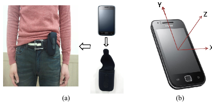
Fig. 1. (a) The direction in which the smartphone is inserted into its case and the position of its attachment on the body of the subject. (b) The direction of each axis on the smartphone.
