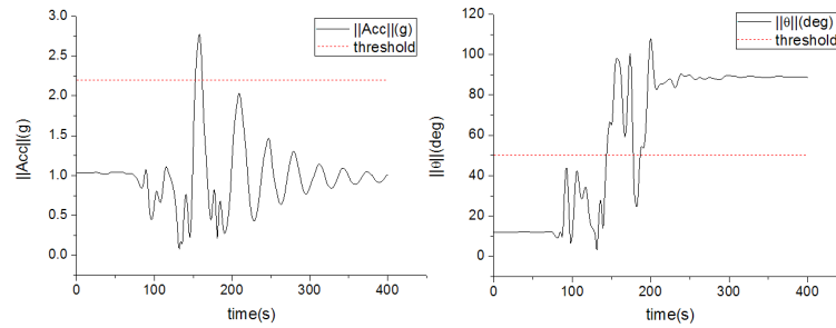
Fig. 2. Results of forward falls.
