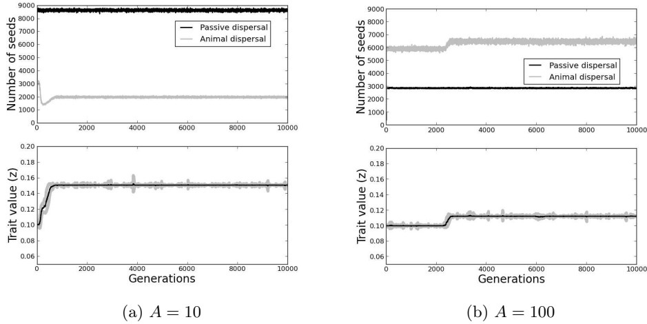
Fig. 5: Trait evolution ( z ) and proportion of passive and frugivore dispersed seeds under two scenarios of frugivore abundance A using cheap fruit costs ( \theta = 2 ): a) low abundance ( A = 10 ) and b) high abundance ( A = 100 ). Decreasing animal abundance promotes the evolution of frugivory. For parameters values used see Table 1.
