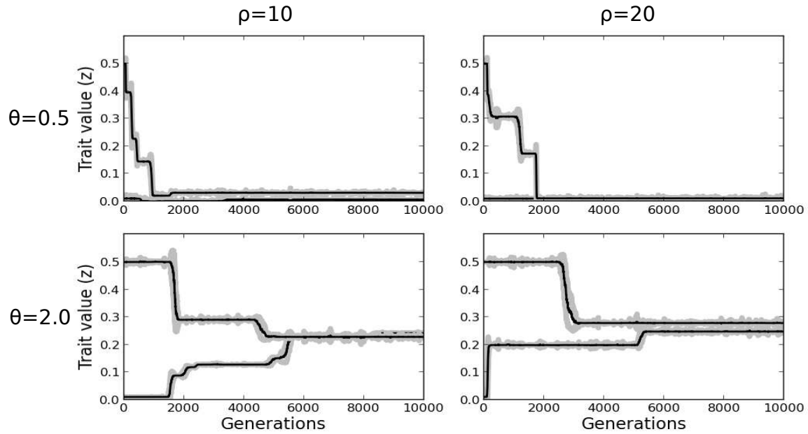
Fig. 3: Typical trait evolution for two different initial conditions under different values of the cost parameter \theta and frugivore choosiness \rho . Black lines correspond to the mean trait in the population and gray lines to the standard deviation. Fruit production costs and choosiness have an important effect on the evolution of frugivory. Costly fruits do not favor the evolution of frugivory, but choosy frugivores can promote it, especially when costs are low. For parameters values used see Table 1.
