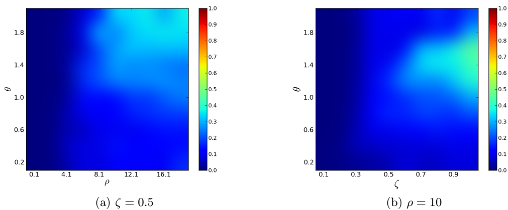
Fig. 4: Average frugivory trait ( \bar{z} ) values as a function of the cost parameter \theta and (a) the frugivore choosiness ( \rho ), and (b) response threshold. \zeta . The average value was taken from ten simulations for each parameter ( \theta, \rho ) and ( \theta, \zeta ) combination. In general, decreasing fruit costs and increasing choosiness ( \rho \gg 0, \zeta > 0.5 ) promote the evolution of frugivory. The initial value of the trait was z_0 = 0.1 . For other parameters values used see Table 1.
