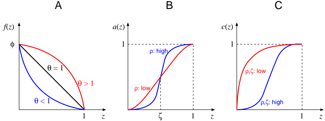
Fig. 2: (A) Trade-off between fruits per tree f , and the trait that promotes frugivory z (e.g. fruit size or pigmentation). The parameter \theta is inversely related with the cost of the trait, e.g. \theta > 1 "cheap" (red solid line), \theta < 1 "costly" (blue solid line). (B) Fruit consumption rate a as a function of the trait z . The shape parameter \rho ( \rho_{low} = 5 , \rho_{high} = 20 ) measures the frugivore's choosiness: the higher the \rho the steeper the curve and the choosier the frugivores. \zeta is the response threshold of the frugivores. (C) Probability c that a fruit is eaten by a frugivore as a function of the trait value z . A high and low \rho curve is shown as a blue and red solid line, respectively.
