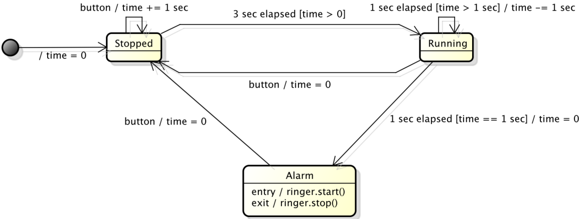
Figure 3.5: The UML state machine diagram modeling the dynamic behavior of the countdown timer application.
