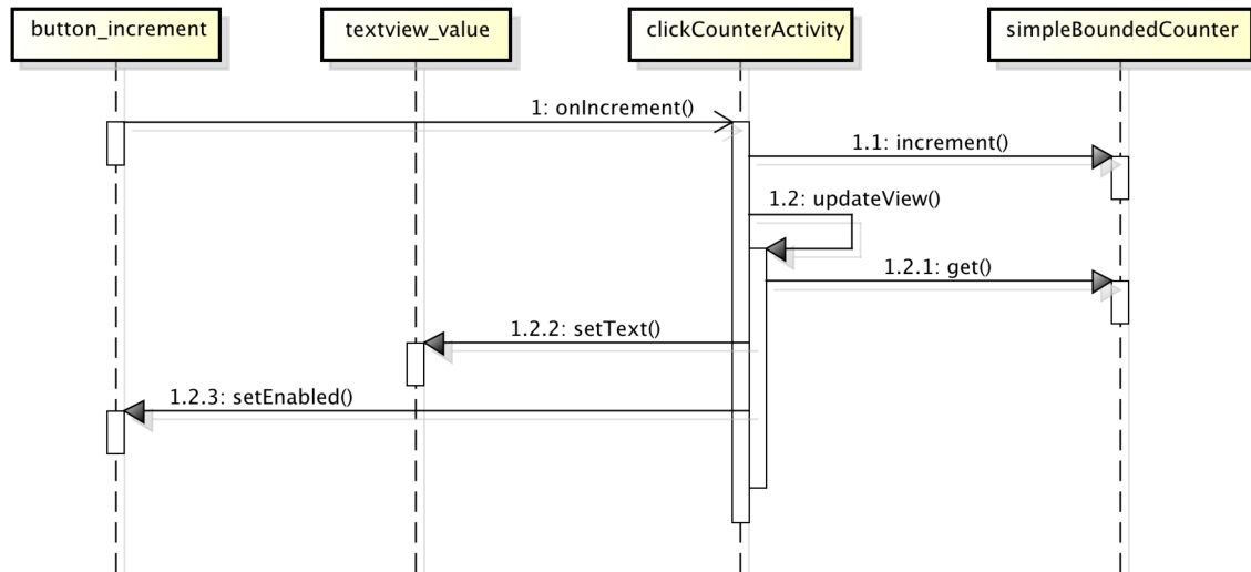
Figure 2.8: This UML sequence diagram shows the full event-based interaction cycle in response to a press of the increment button. Stick arrow heads represent events, while solid arrow heads represent method invocations.
