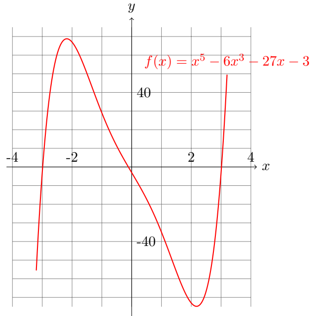
Figure 23.4. The graph of f(x) = x^5 - 6x^3 - 27x - 3
