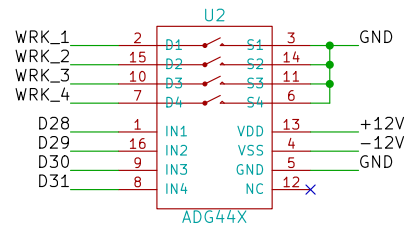
Multiplexing for working electrodes 1-4
