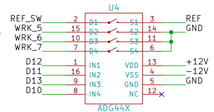
Multiplexing for working electrodes 5-7 plus switches for counter and reference electrodes
