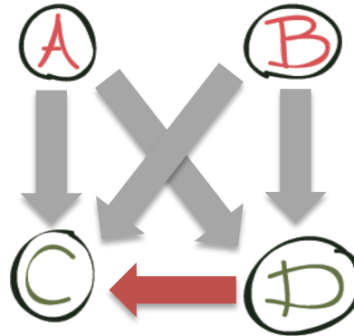
Dependence modeled by DAG
