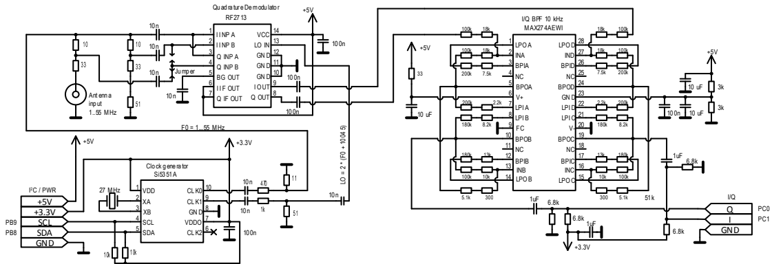
EU1KY Antenna analyzer V2 1..55MHz RF frontend
