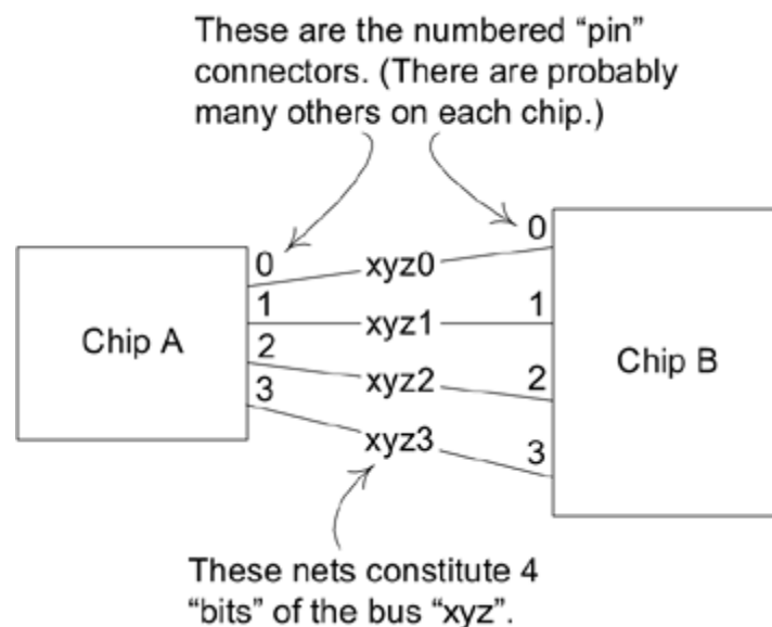
Figure 3.2. An explanatory diagram of buses and nets
