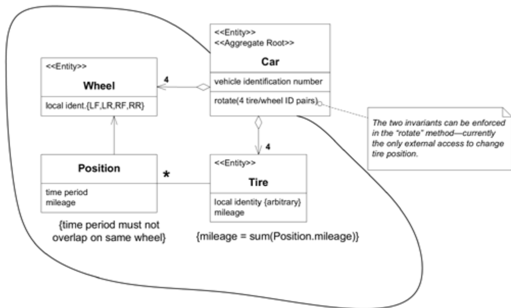
Figure 6.3. AGGREGATE invariants
